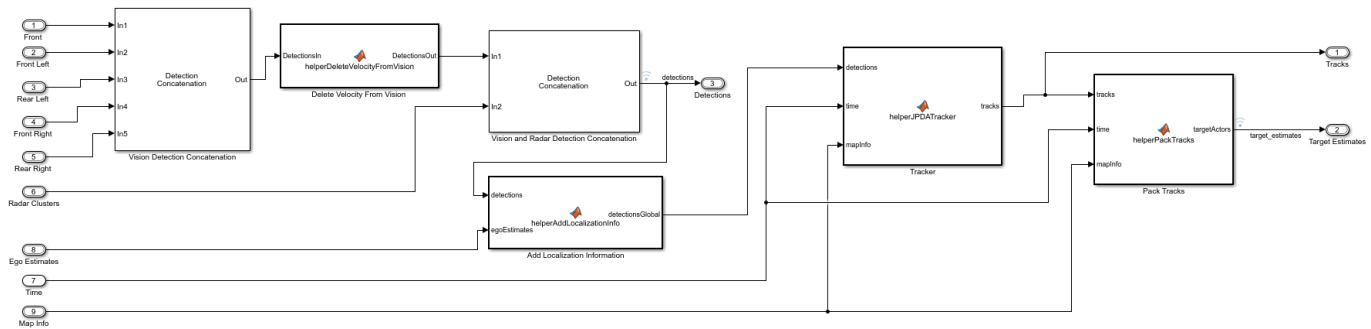
Surround Vehicle Sensor Fusion
